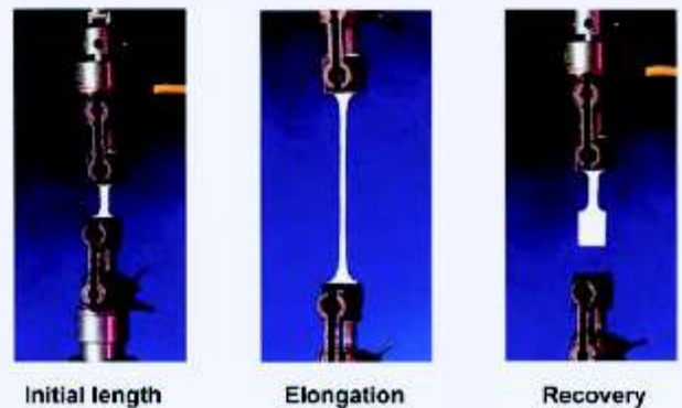
Fig. 1 Elongation and Recovery according to: ASTM D 412
