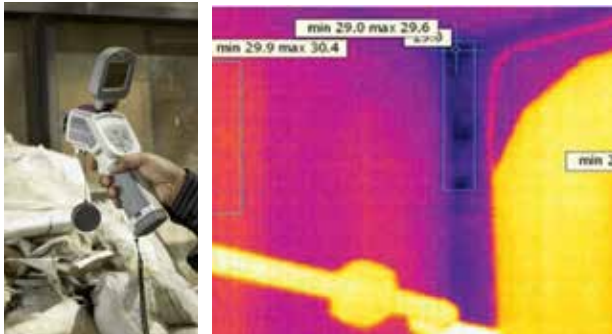
IR Thermography to detect delamination and voids of concrete as well to find out the source of water leakage and location of water pipe
