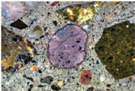
Fig. 7: Reacted particles are identified by dark areas that indicate ASR gel (either inside the particle, or along edges of particles)
