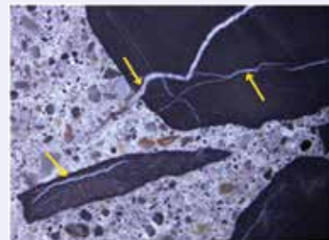
Fig. 10: Stereo-optical photo-micrograph of polished concrete specimen showing alkali-silica reaction (ASR) gel filled cracks extending from reactive aggregate into the cement paste
