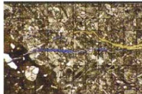
Fig. 12: Microscopic view of alkali-carbonate reactive aggregates
