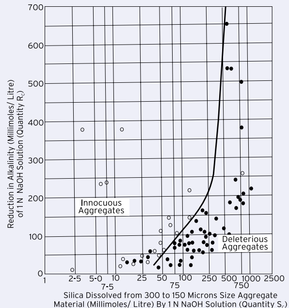
Fig. 9: Illustration of division between innocuous and deleterious aggregates on bases of reduction in alkalinity
